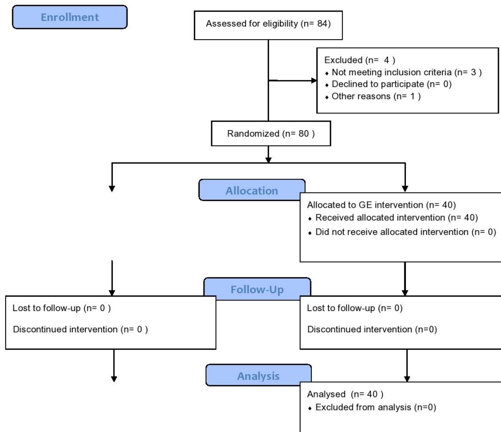
Figure 1: Participant Flowchart
